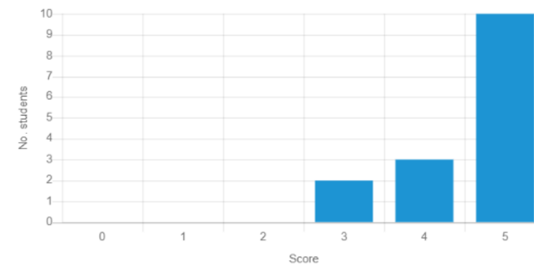
Score distribution
